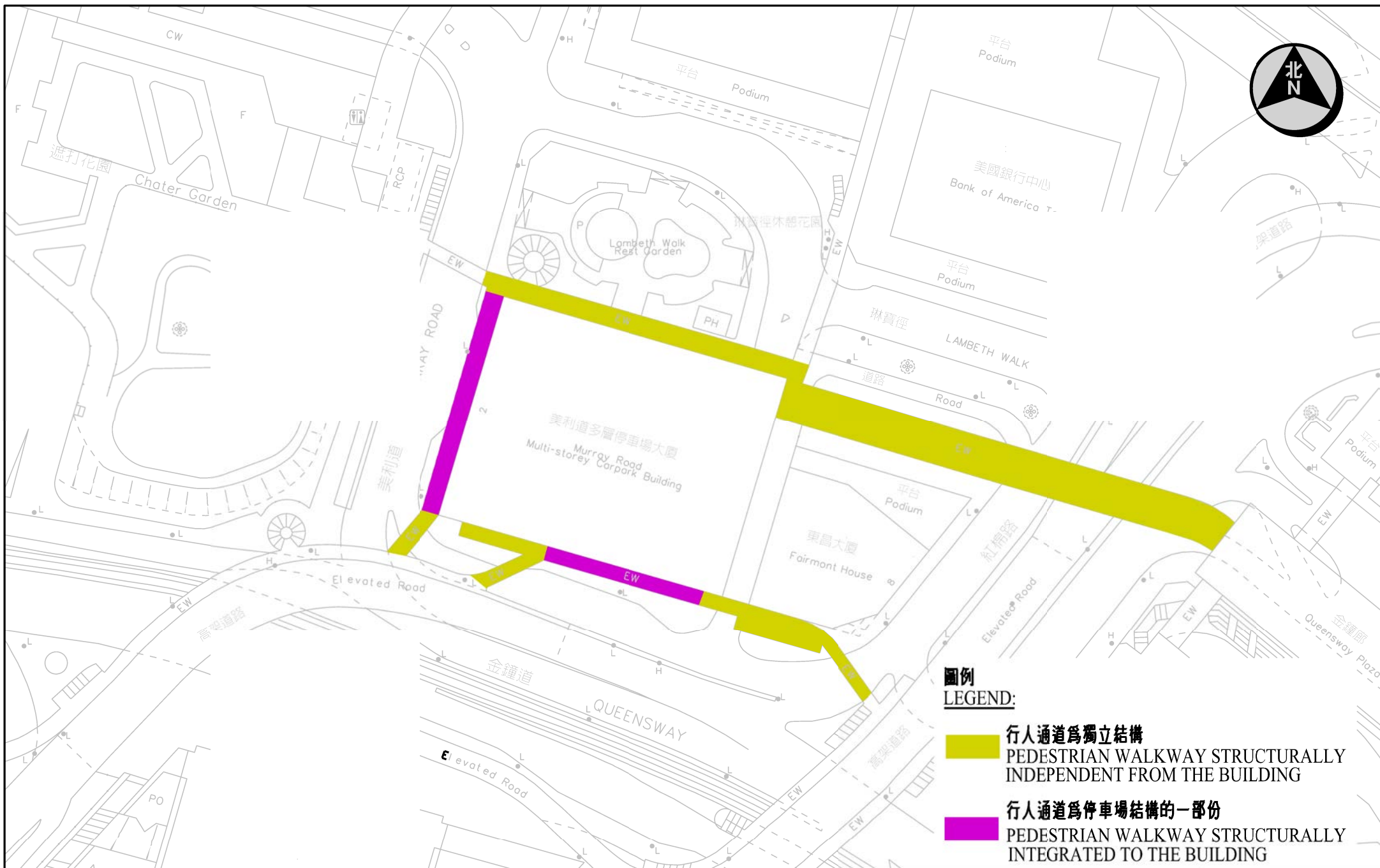
圖一 - 美利道多層停車場旁現時的行人通道 PLAN 1 - EXISTING ELEVATED PEDESTRIAN WALKWAY ADJACENT TO MURRAY ROAD MULTI-STOREY CARPARK
