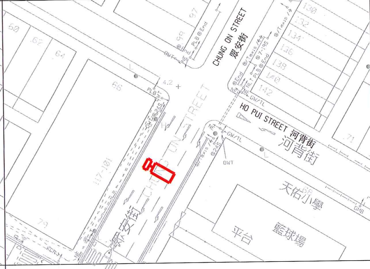
PROPOSED DWF1 AT CHUNG ON STREET 擬建造的旱季截流器 - 眾安街
