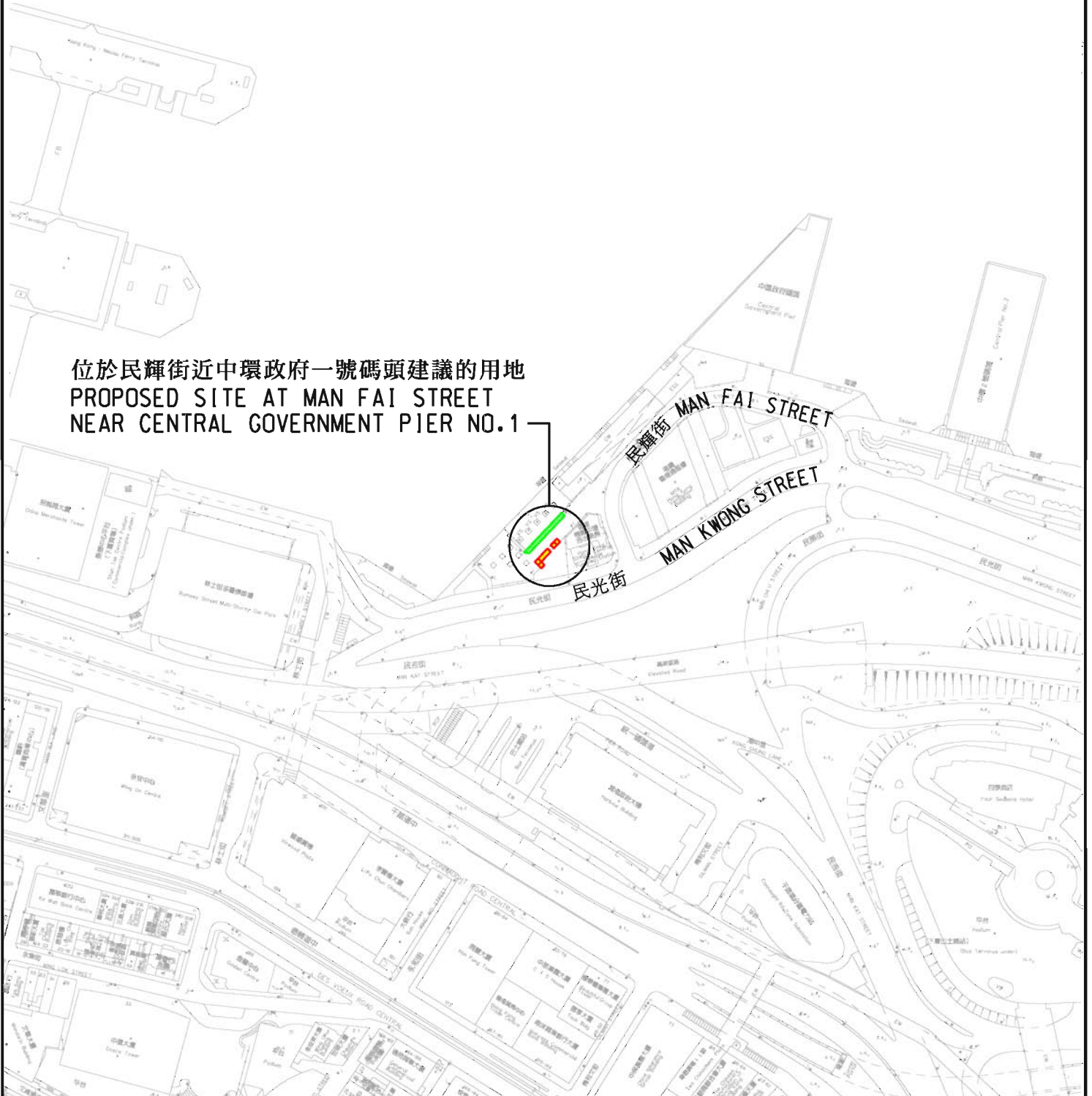
遷置灣仔龍景街五個機動船亭至中環民輝街 - 位置圖 RELOCATION OF 5 MOTOR BOAT KIOSKS FROM LUNG KING STREET (WANCHAI) TO MAN FAI STREET (CENTRAL) - LOCATION PLAN
