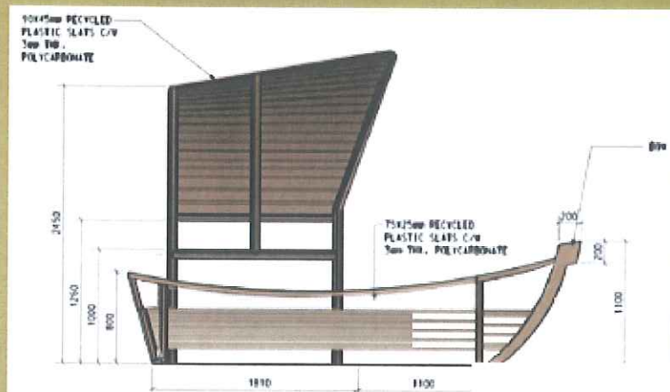
Sampan Seating Elevation 舢舨立面圖
