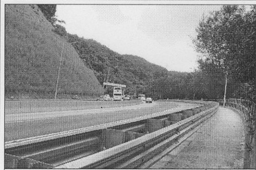
雙層三波護欄 NEW DOUBLE THREE-BEAM BARRIER
