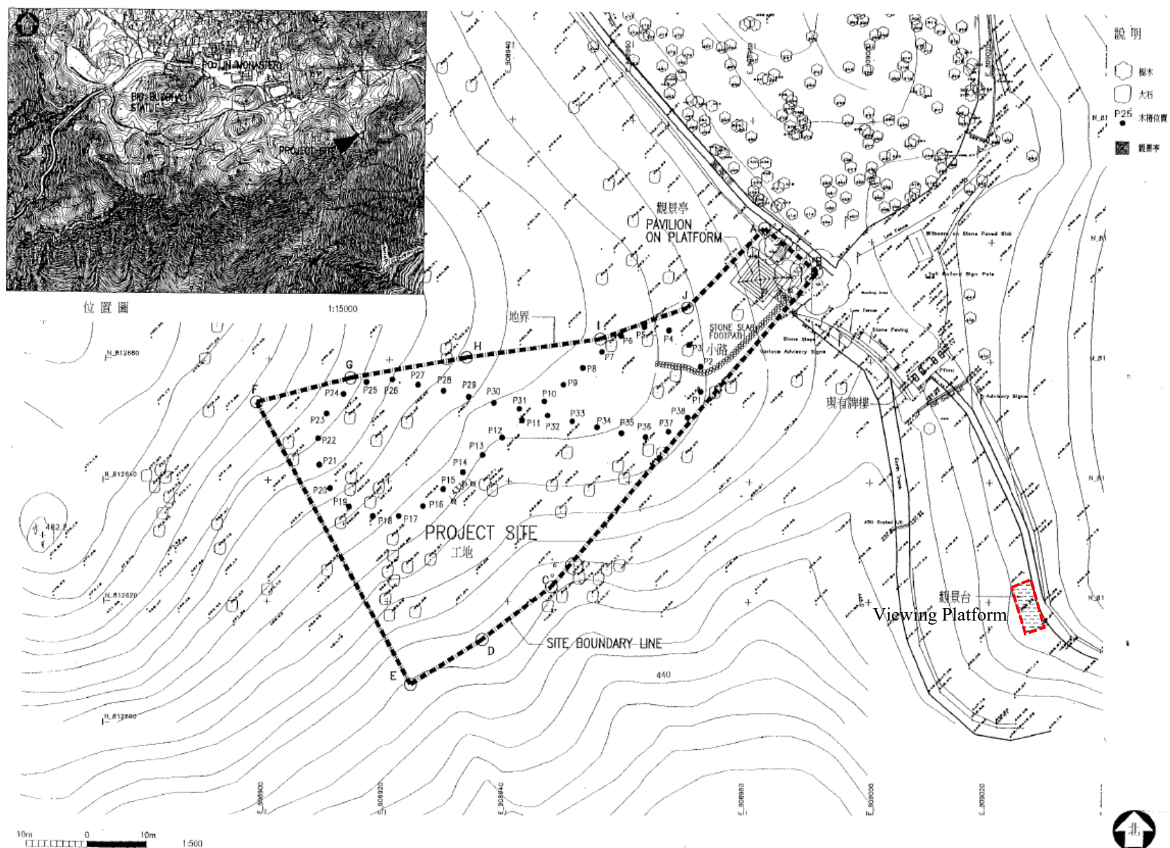
Location plan of viewing platform
