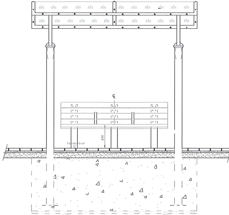
Front view of rain shelter 1:35
