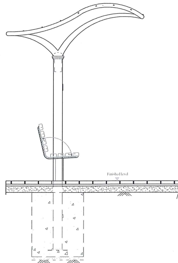
Elevation of rain shelter 1:35
