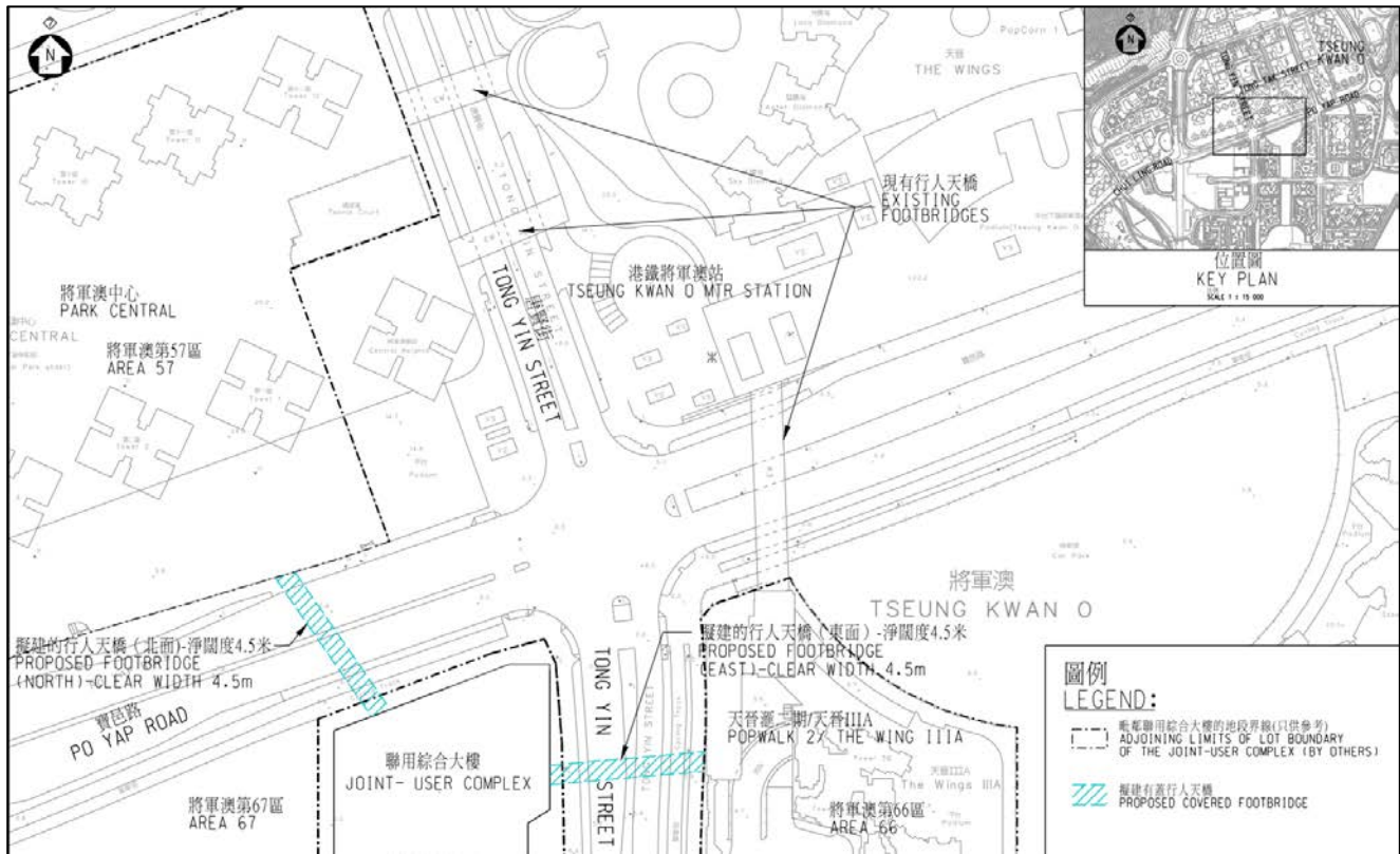
Layout Plan
