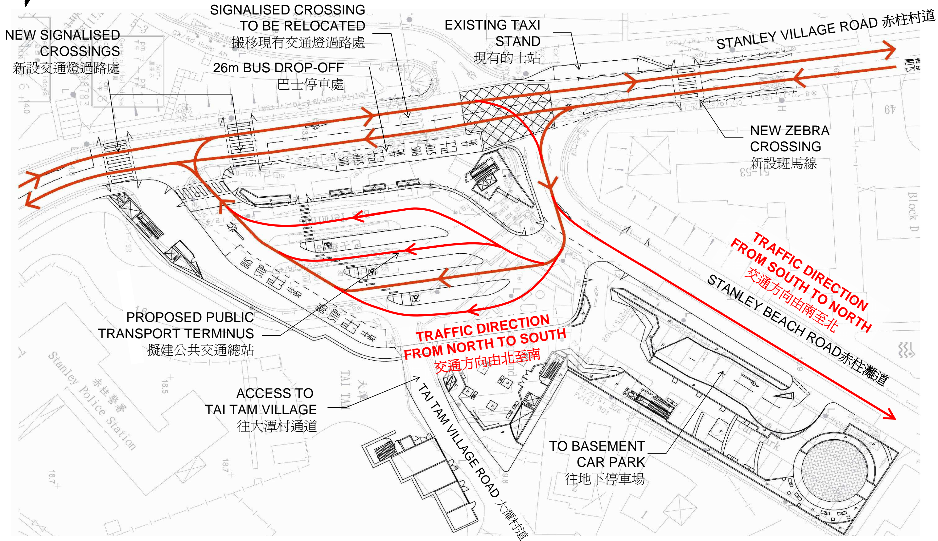
73TI – Multi-storey Carpark and Public Transport Terminus at Stanley Village Road
