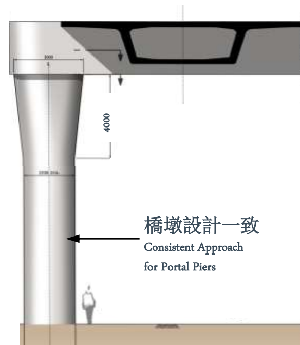
橋墩正面圖 Front Elevation at Portal
