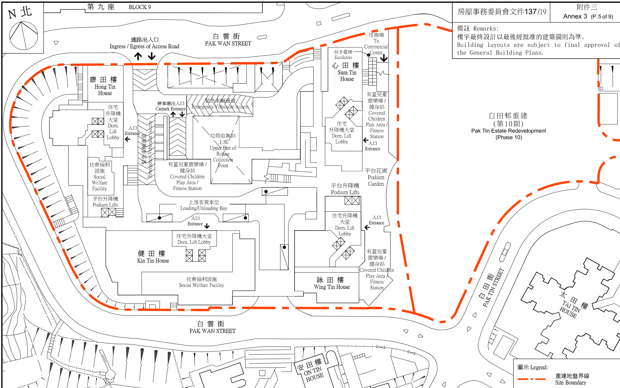
白田邨重建(第7及8期)地下概念圖 Pak Tin Estate Redevelopment (Phases 7 & 8) G/F Conceptual Layout
