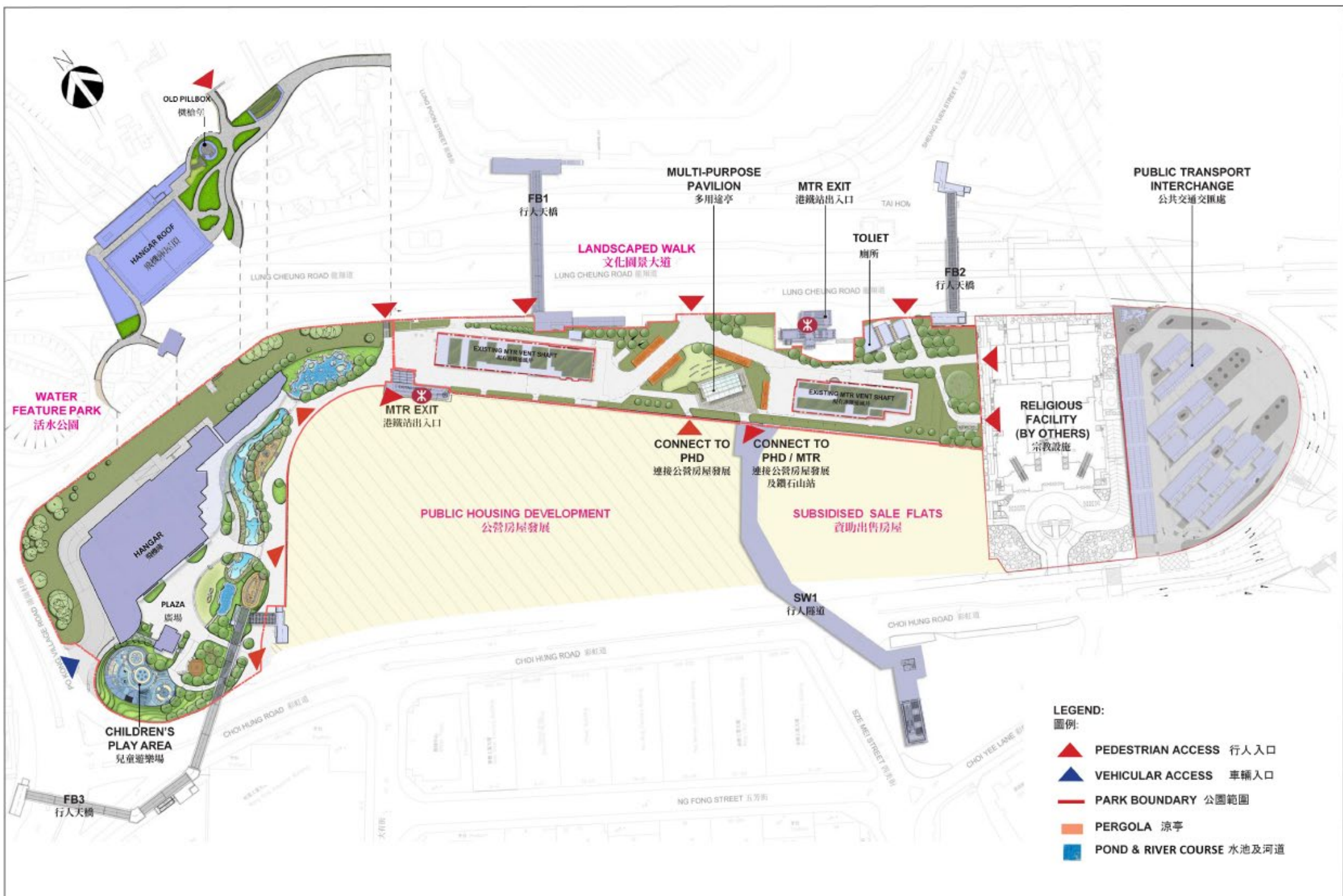
WATER FEATURE PARK AND LANDSCAPED WALK OVERALL DESIGN
