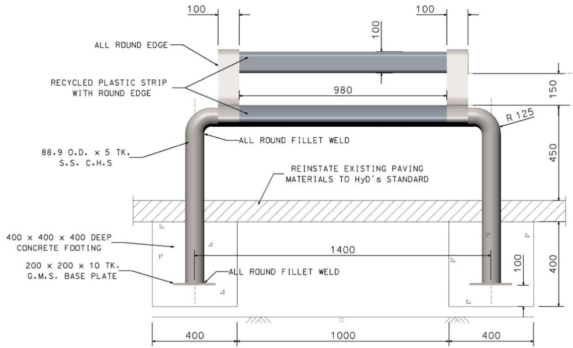
Front View
